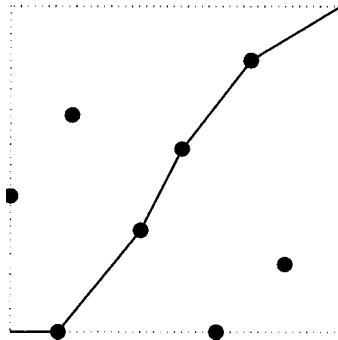
Fig. 1. A points selection and the longest up/right path.
